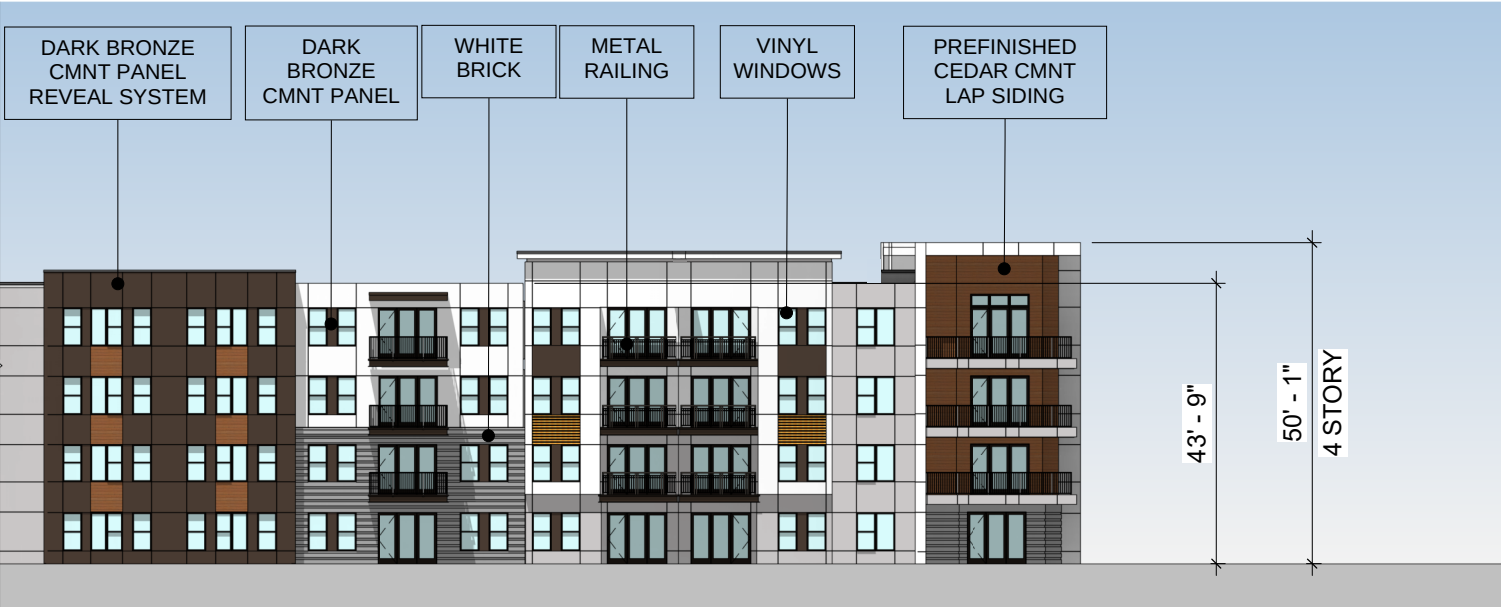
2. BUILDING 300 - EAST ELEVATION B
