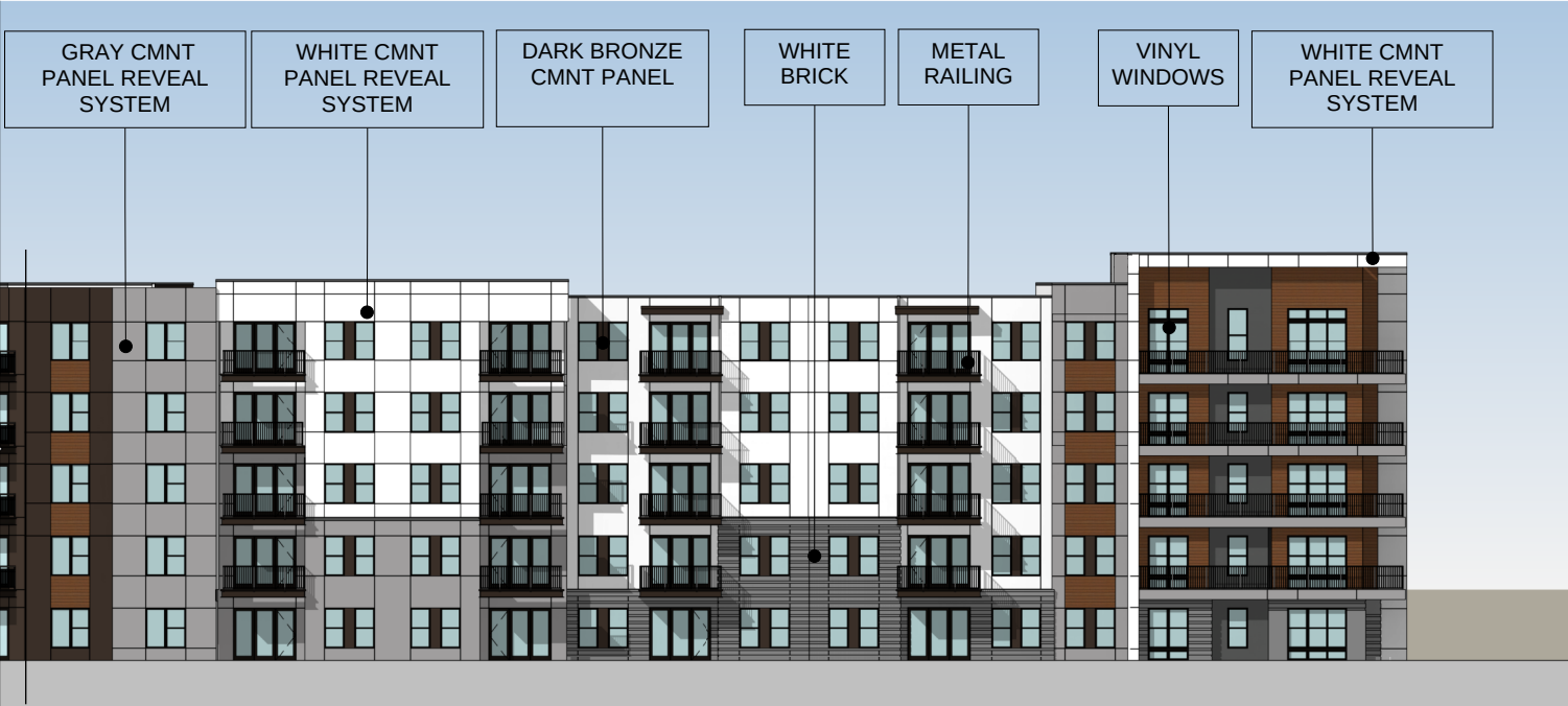
2. BUILDING 300 - EAST ELEVATION B
